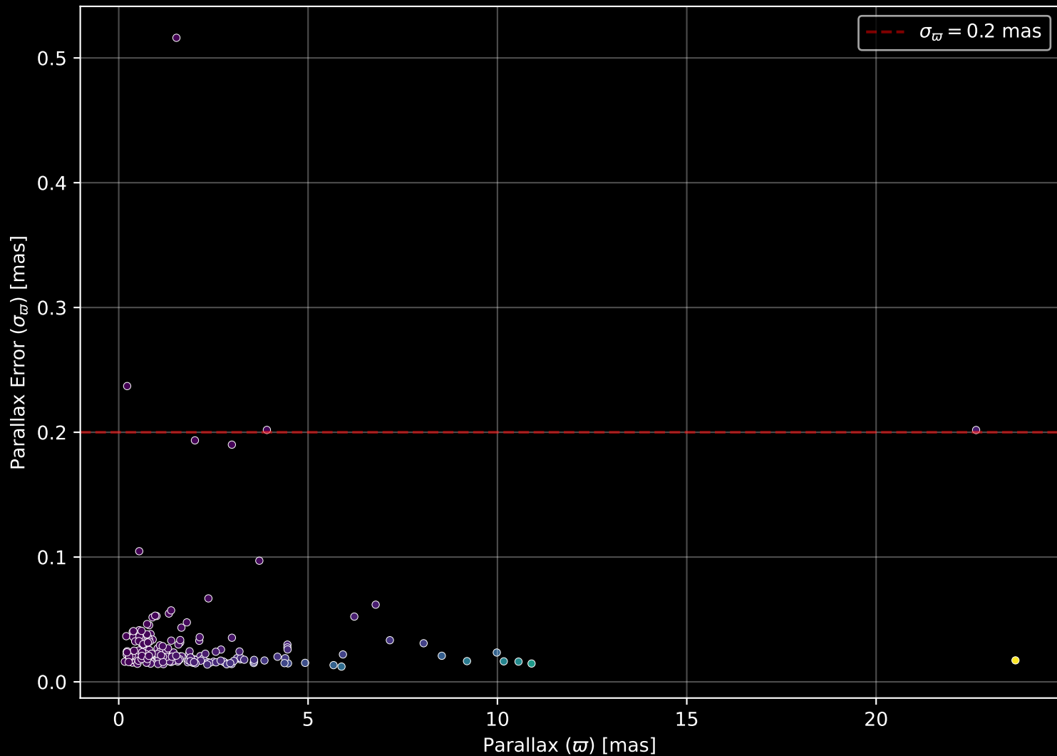
APOGEE DR17 Field: [K2_C13_180-15_btx] Parallax Quality (n= 187)
