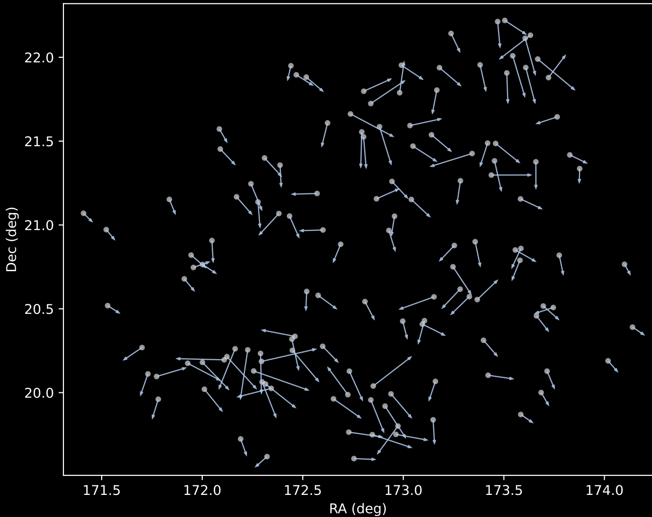
APOGEE DR17 Cluster 1 Proper Motion Vectors (n=130)
