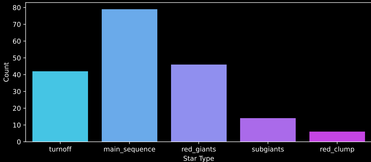
APOGEE DR17 Field: [K2_C13_180-15_btx] Count plot of Star Type
