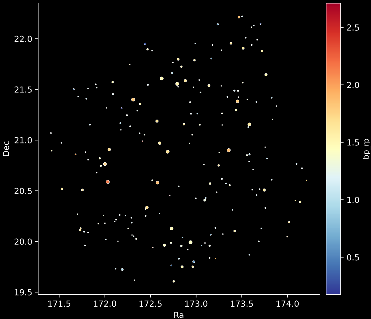
APOGEE DR17 Field: [K2_C13_180-15_btx] Stars: 187
