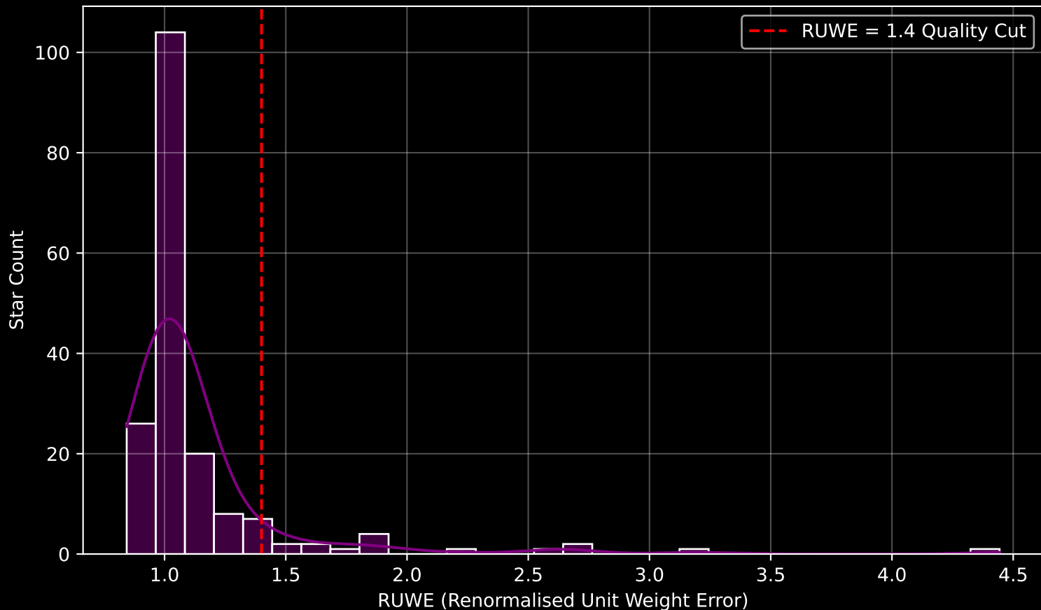
GAPOGEE DR17 Field [K2_C13_180-15_btx] RUWE Distribution (n= 180)
