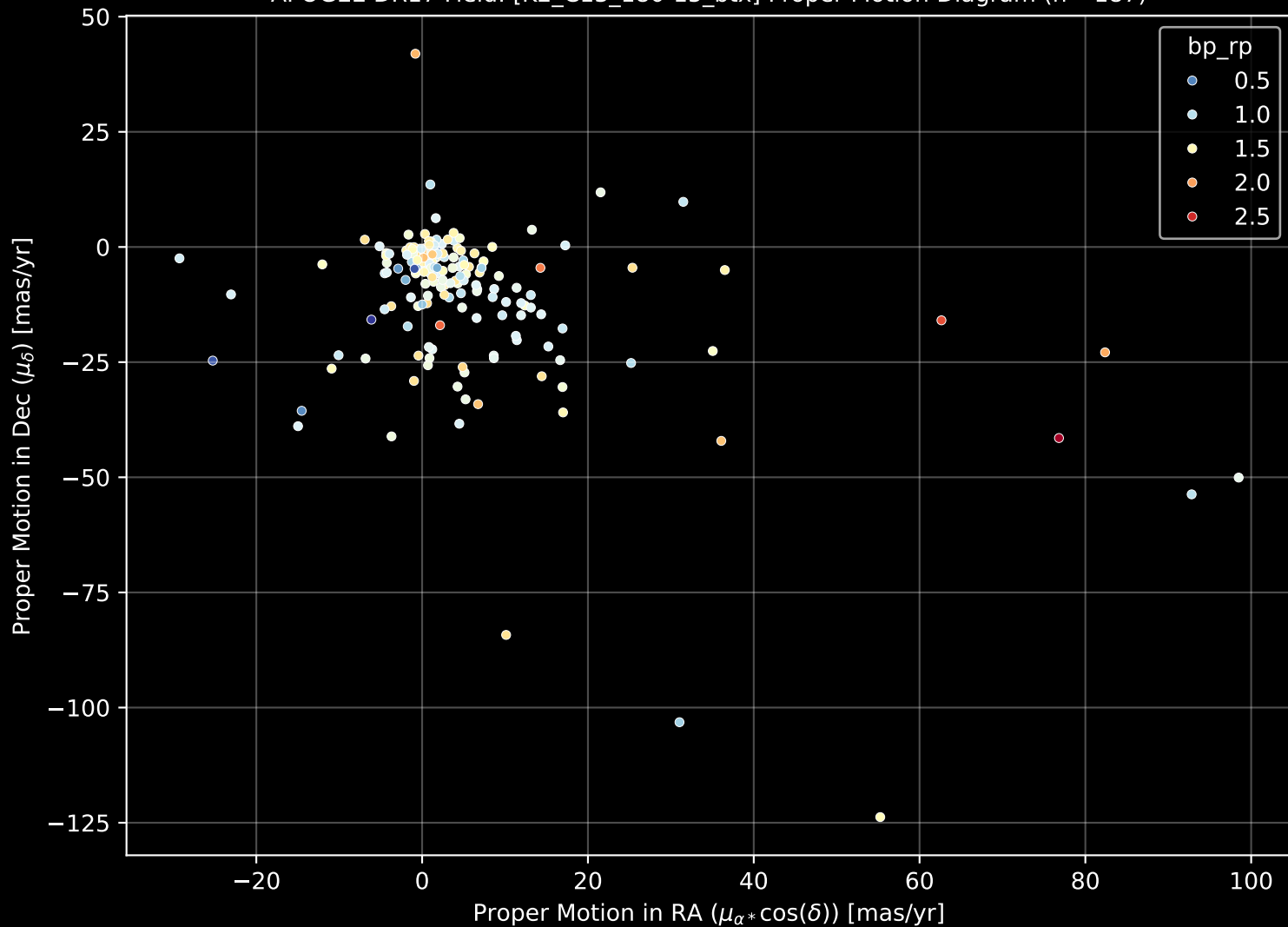
APOGEE DR17 Field: [K2_C13_180-15_btx] Proper Motion Diagram (n= 187)
