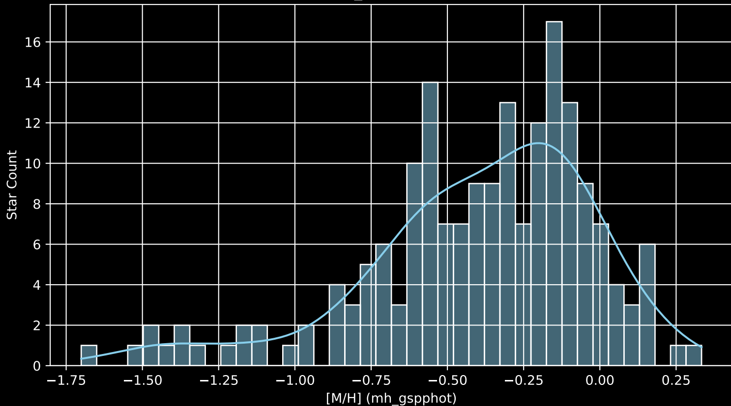
APOGEE DR17 Field: [K2_C13_180-15_btx [M/H] (mh_gspphot) (n= 186)
